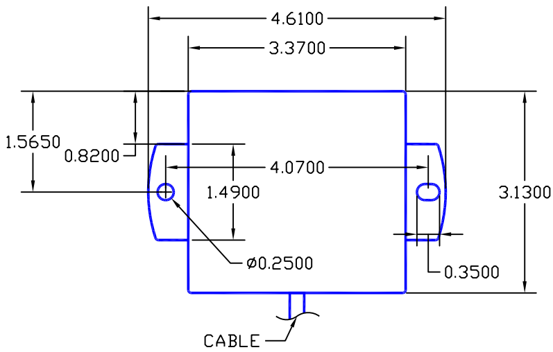
04Y-310 CDI CAPCITIVE DISCHARGE IGNITION
