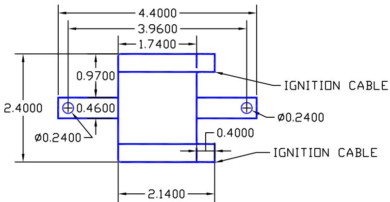
04Y-450 IGNITION COIL ASSEMBLY
