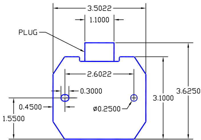
04Y-323 VOLTAGE REGULATOR
